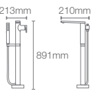
COMPOSED™ | K-73087T-B4-CP Floor mount bathtub filler with hand shower in polished chrome
