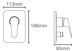
ACCLIV | K-33111IN-4FP-CP
