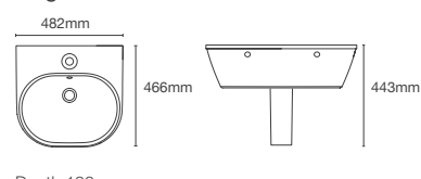
SPAN | K-24560IN-0
