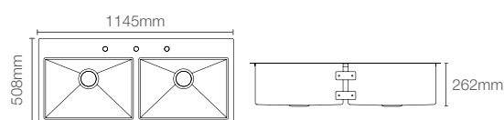
STRIVE™ | K-38807IN-NA
