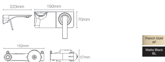
MODERNLIFE EDGE™ | K-29199IN-4ND-RGD
