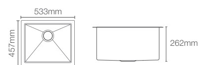
STRIVE™ K-38778IN-NA
