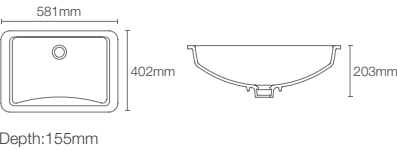
LADENA™ | K-2215IN-2-0
