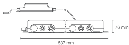
ANTHEM™ | K-28211IN-NA
