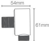
COMPLEMENTARY™ K-22448IN-BL
