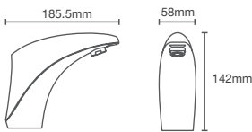
ELOSIS | K-18078IN-ND-CP Touchless cold only basin faucet in polished chrome
