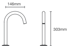
COMPONENTS TALL | K-39558IN-ND-CP Touchless cold only tall sensor faucet in polished chrome
