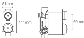
AQUA TURBO 230 | K-75201IN-CP
