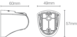
COMPLEMENTARY™ K-99035IN-BL
