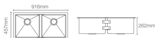
STRIVE™ | K-38801IN-NA
