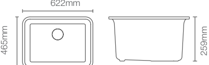
CAIRN R | K-28001IN-CM1 | Matte Black
